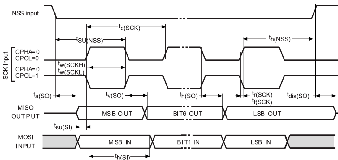
Figure 16. SPI timing diagram - target mode and CPHA = 0
