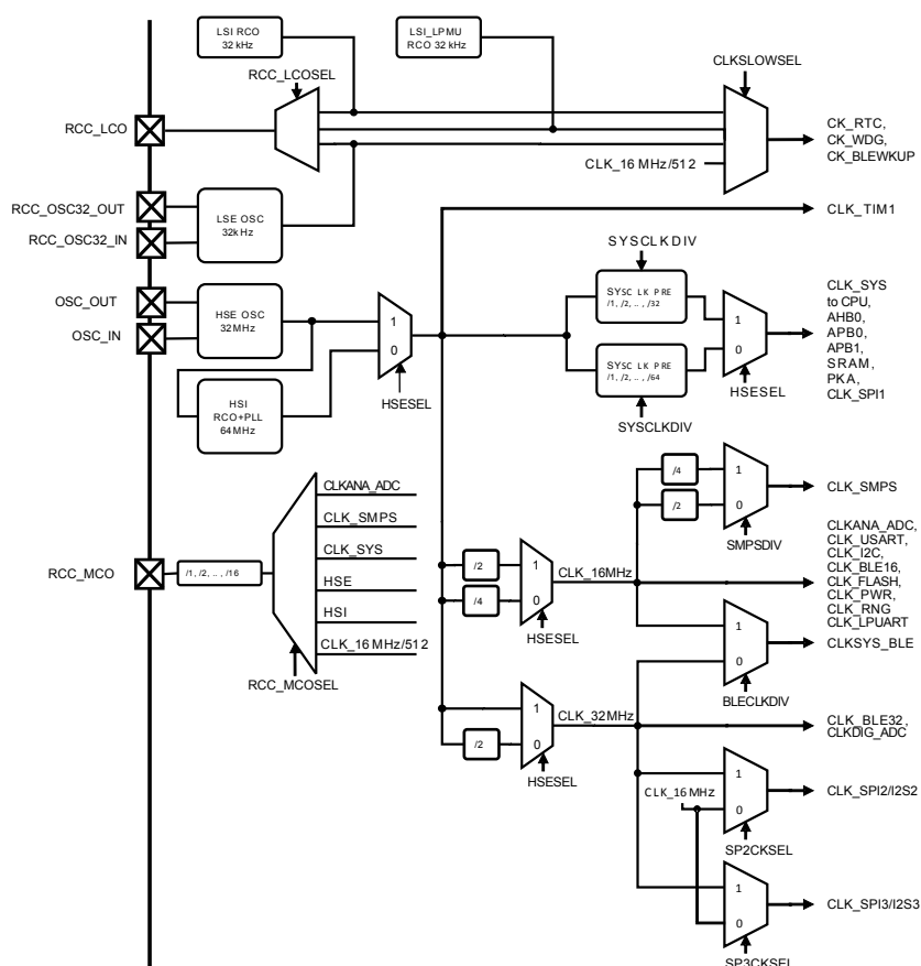
Figure 6. Clock tree
