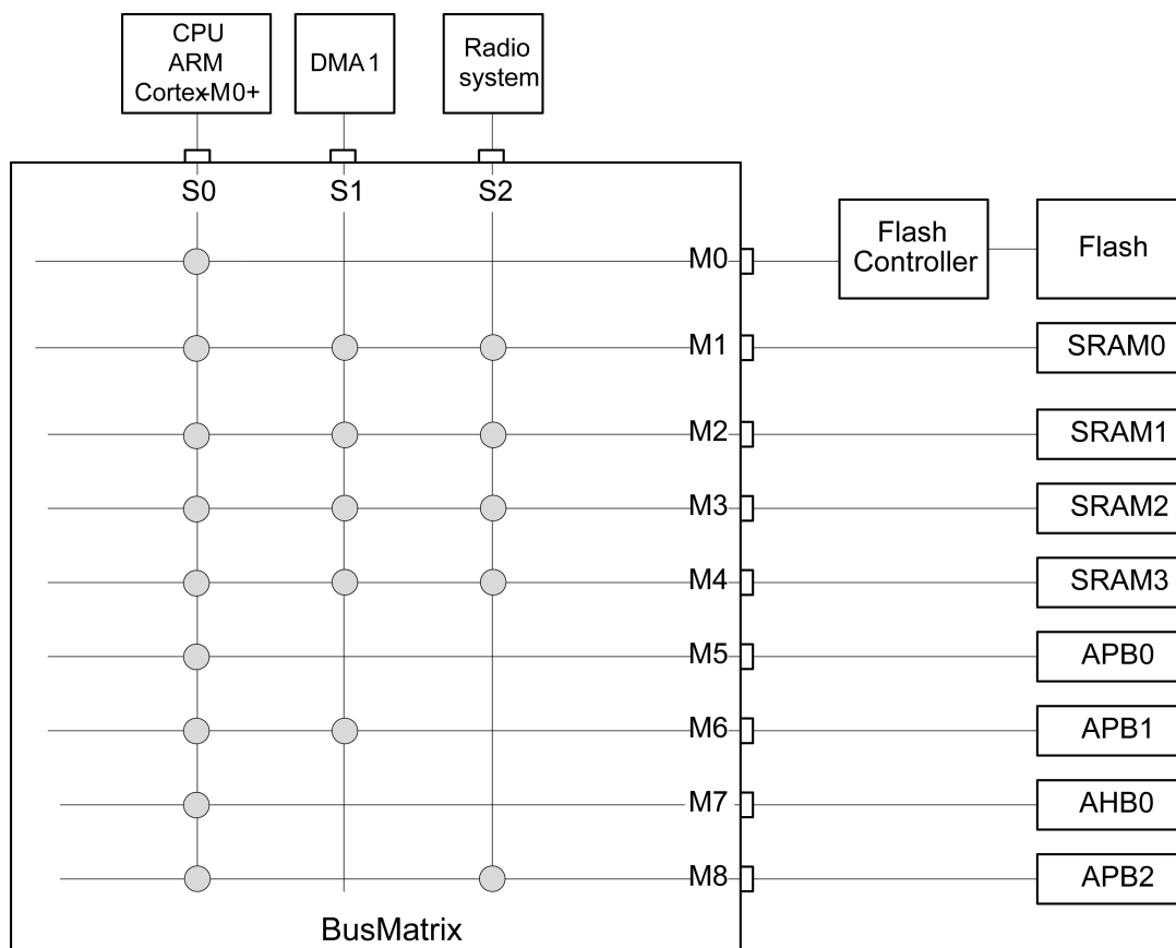
Figure 5. Bus matrix
