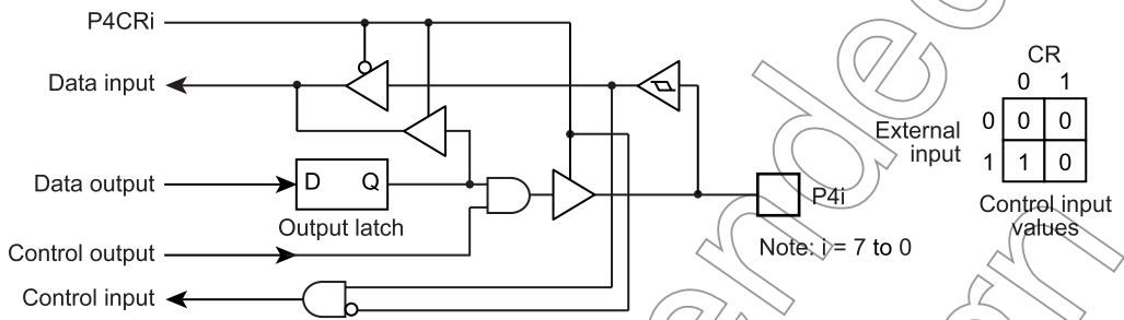
Figure 5-5 Port P4
