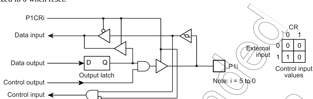
Figure 5-2 Port P1
