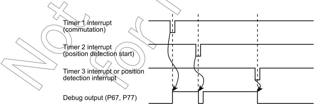
Figure 12-8 DBOUT Debug Output Diagram
