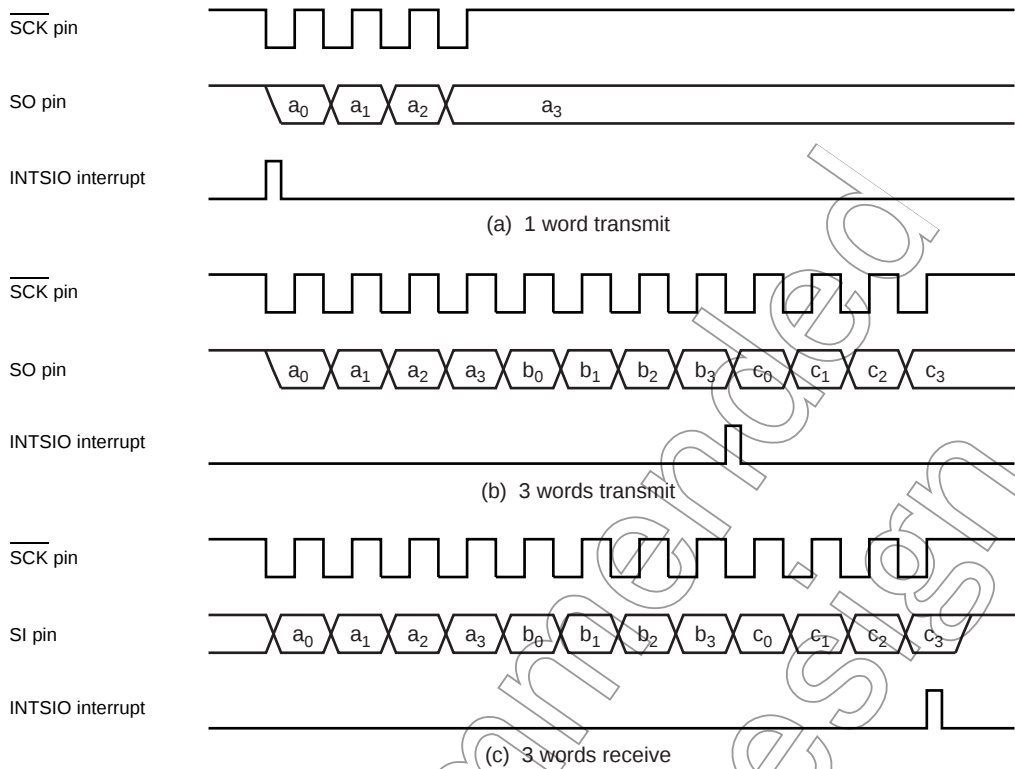
Figure 14-6 Number of words to transfer (Example: 1word = 4bit)
