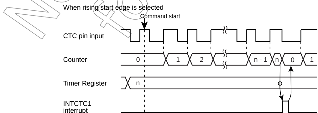
Figure 9-5 Event Counter Mode Timing Chart
