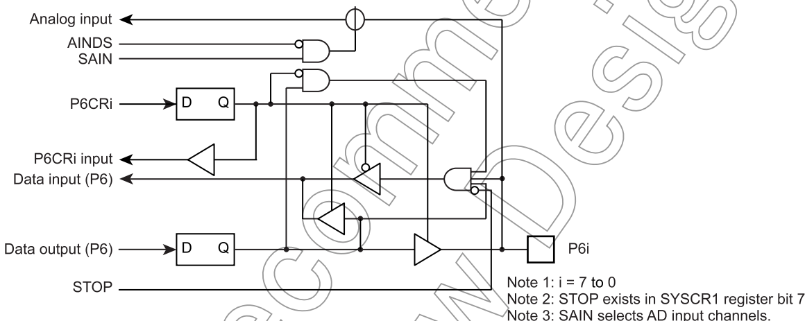
Figure 5-6 Port P6
