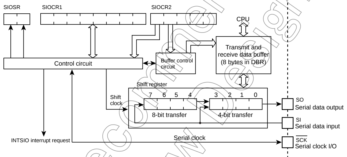
Figure 14-1 Serial Interface
