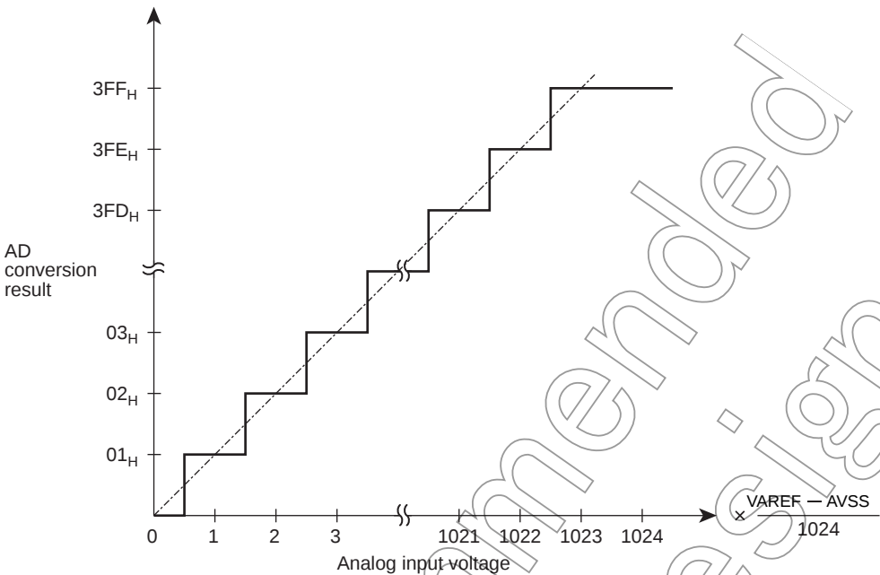
Figure 15-4 Analog Input Voltage and AD Conversion Result (Typ.)
