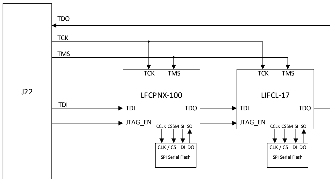
Figure 3.1. Programming Block
