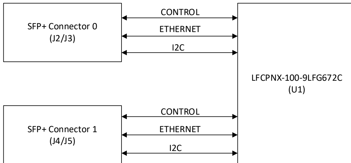
Figure 4.2. SFP+ Interface
