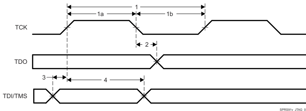
Figure 6-24. JTAG Timing
