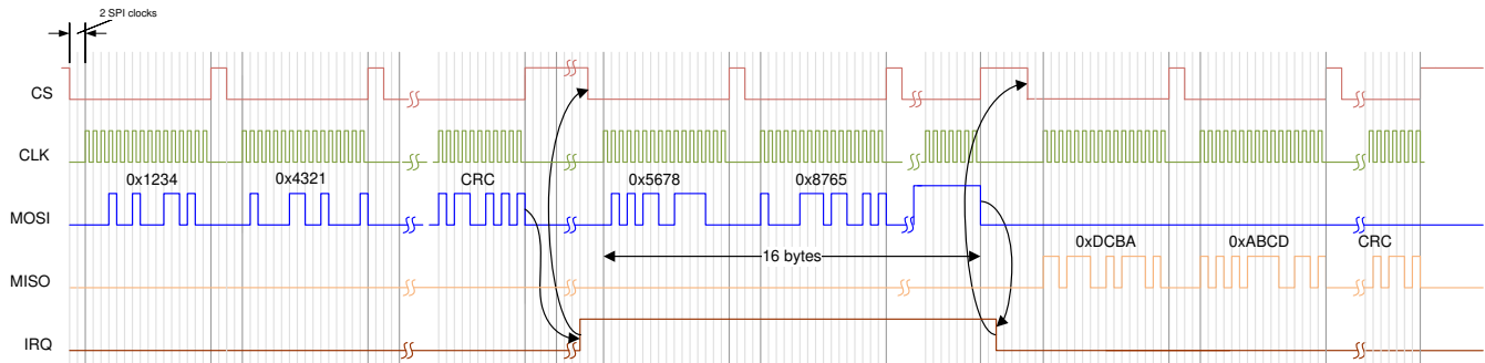
Figure 6-14. SPI Communication
