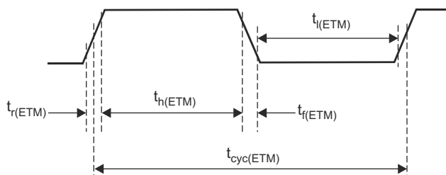
Figure 6-20. ETMTRACECLKOUT Timing
