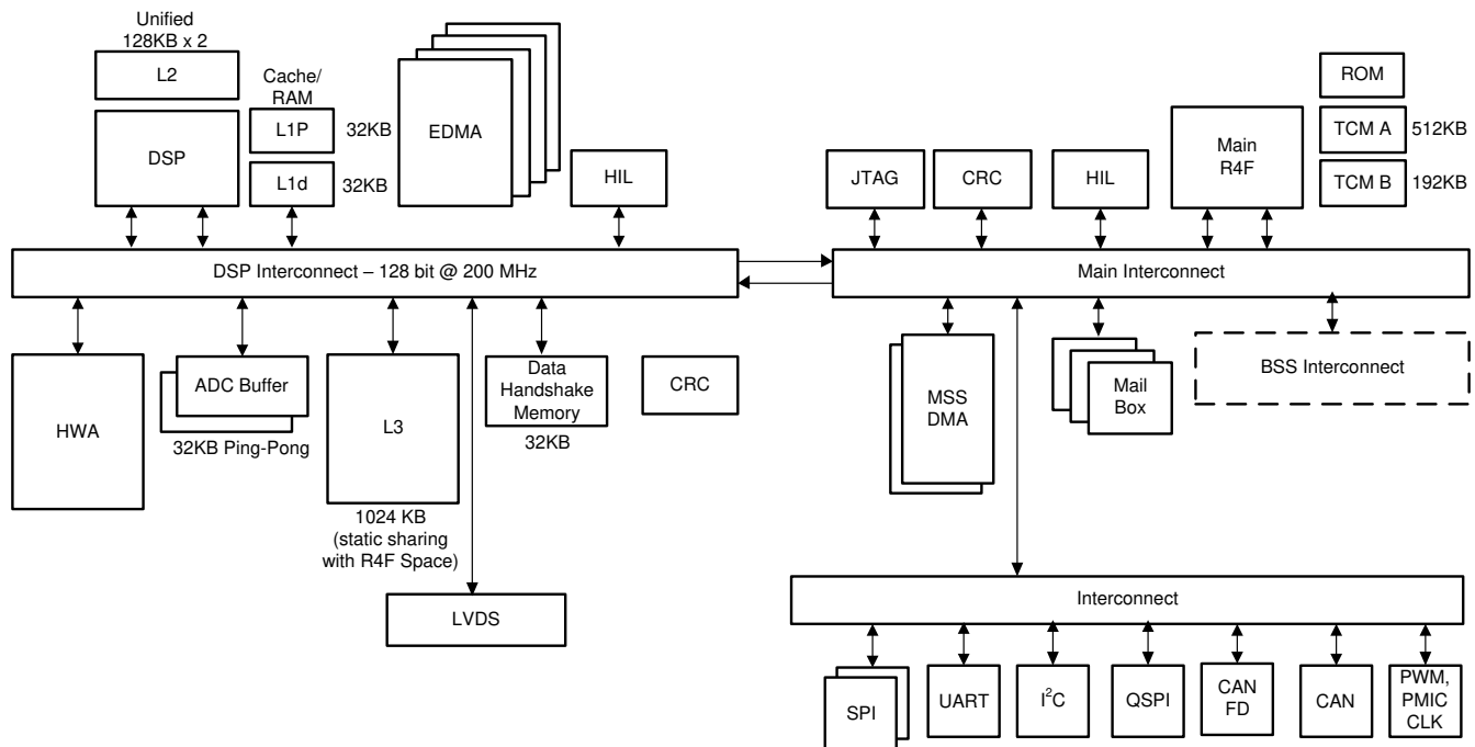
Figure 7-4. Processor Subsystem
