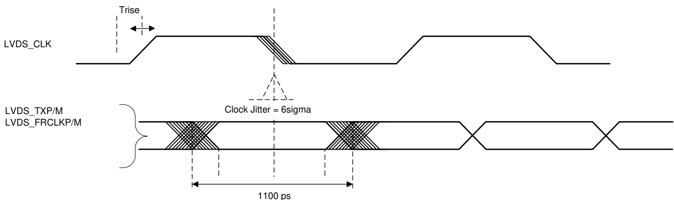
Figure 6-16. Timing Parameters
