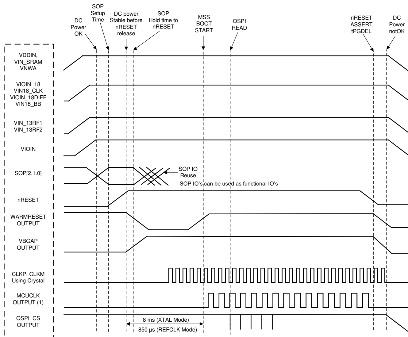
Figure 6-6. Device Wake-up Sequence
