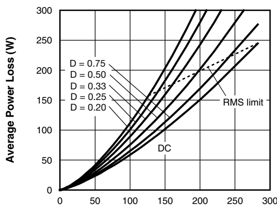
Fig. 6 - Forward Power Loss Characteristics (Per Leg)
