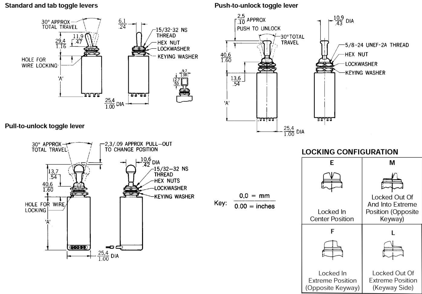
Figure 1. Standard Dimensions
