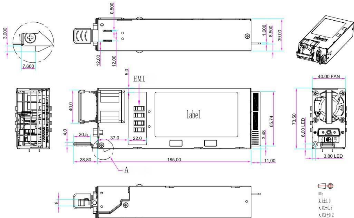
Figure 5. Mechanical Drawing
