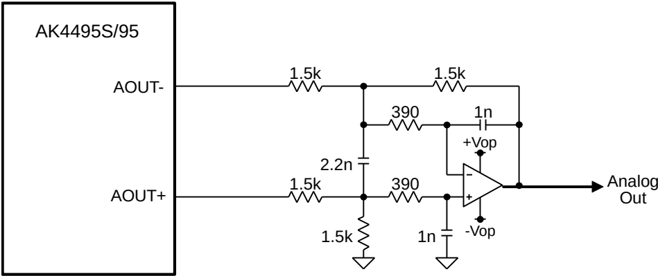
Figure 38. External LPF Circuit Example 1 for PCM ( f_c = 99.2\text{kHz} , Q=0.704 )
