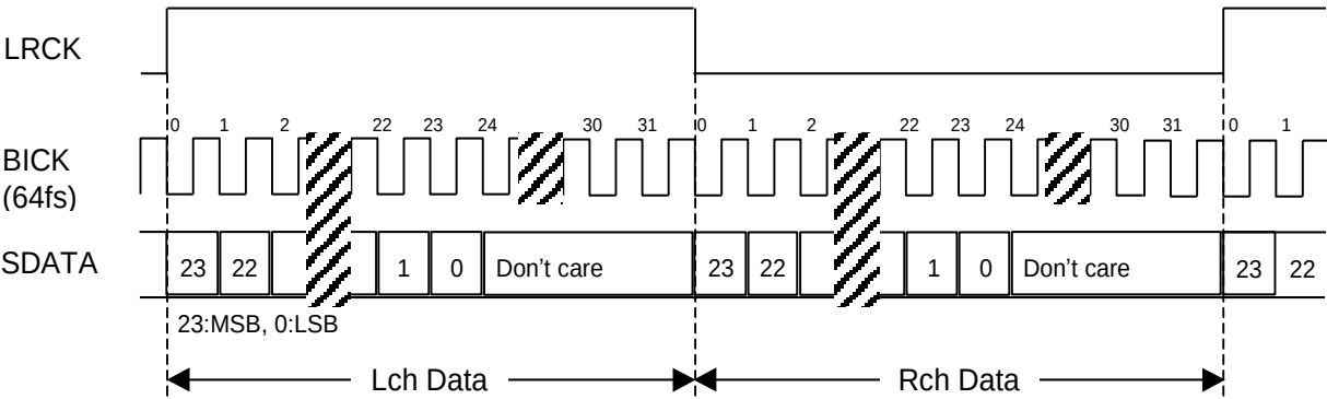
Figure 11. Mode 2 Timing
