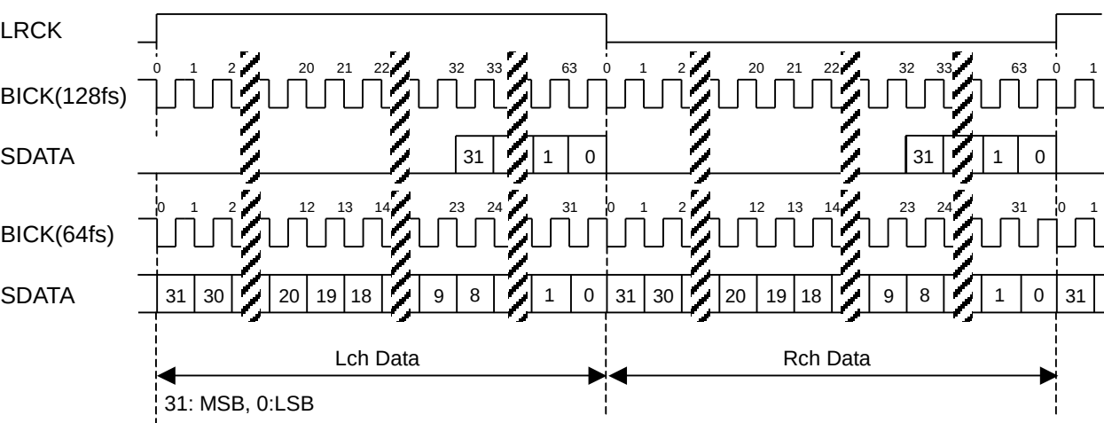
Figure 13. Mode 5 Timing
