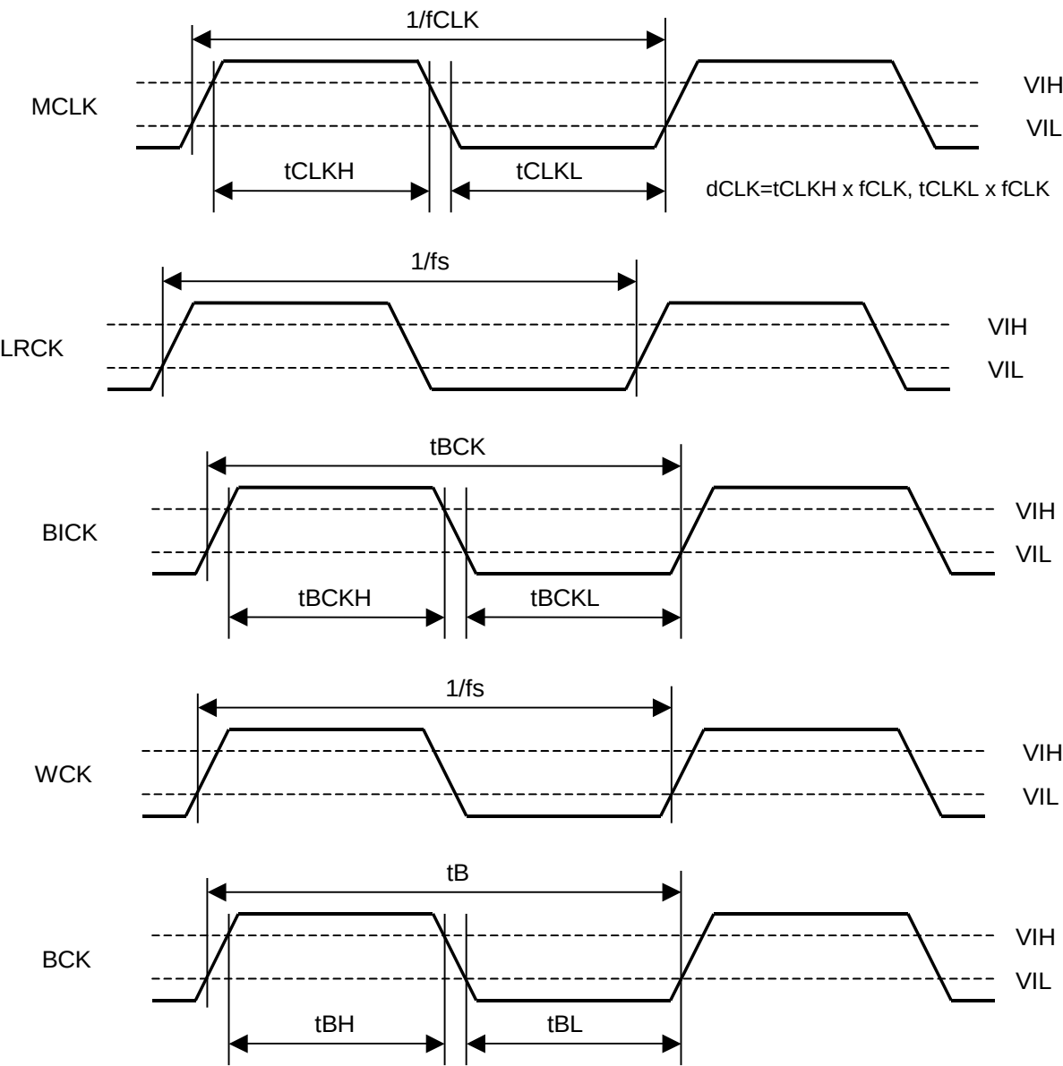
Clock Timing
