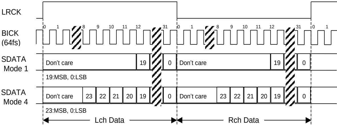
Figure 10. Mode 1/4 Timing
