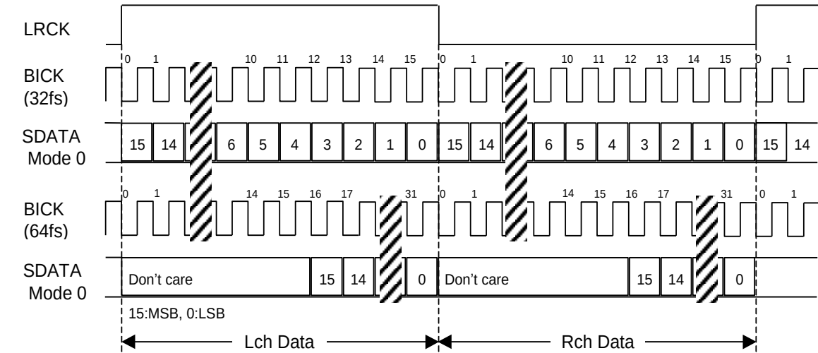
Figure 9. Mode 0 Timing
