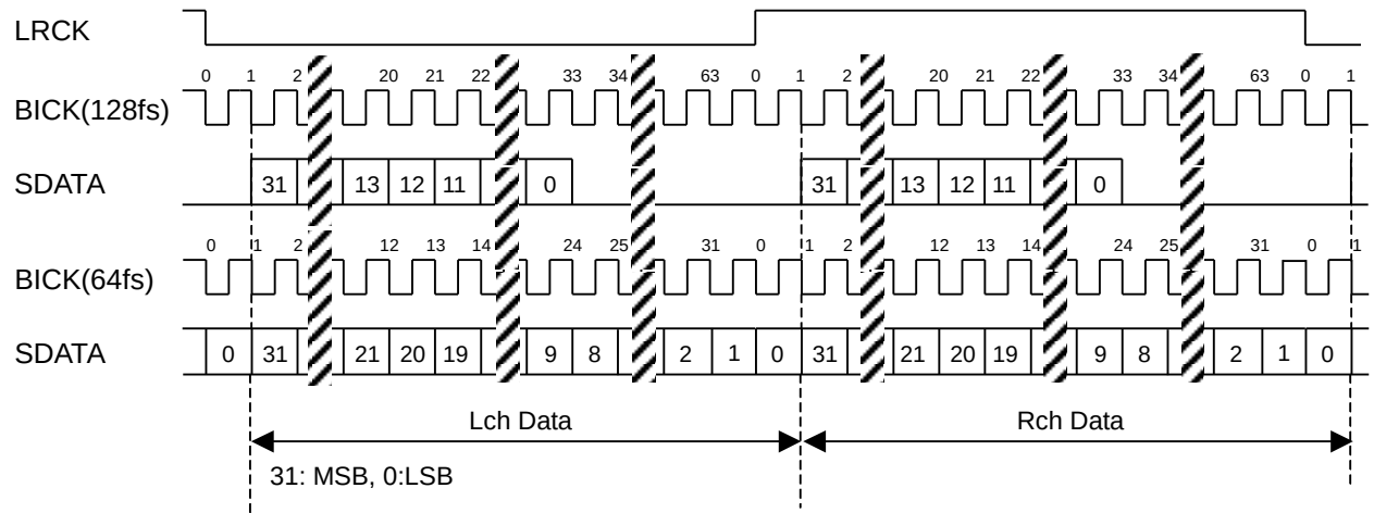
Figure 15. Mode 7 Timing
