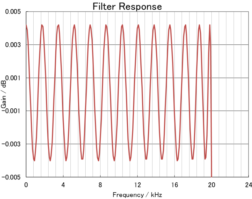
Figure 4. Short Delay Sharp Roll-off Filter Passband Ripple
