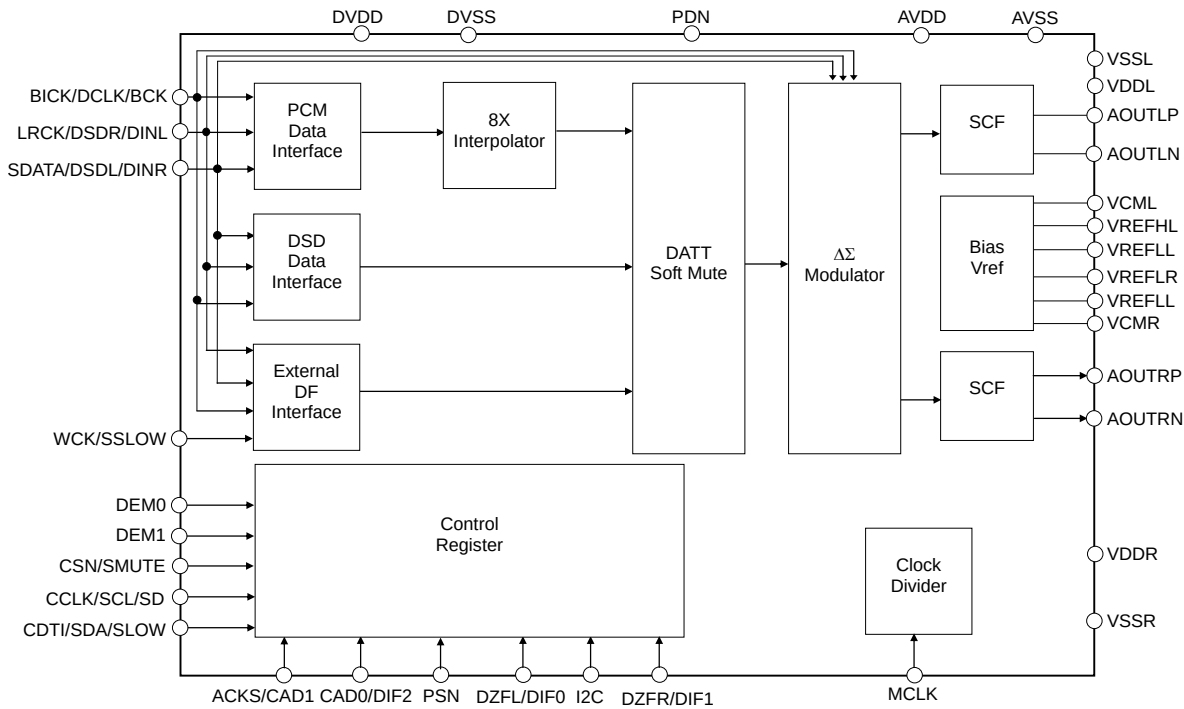
Block Diagram
