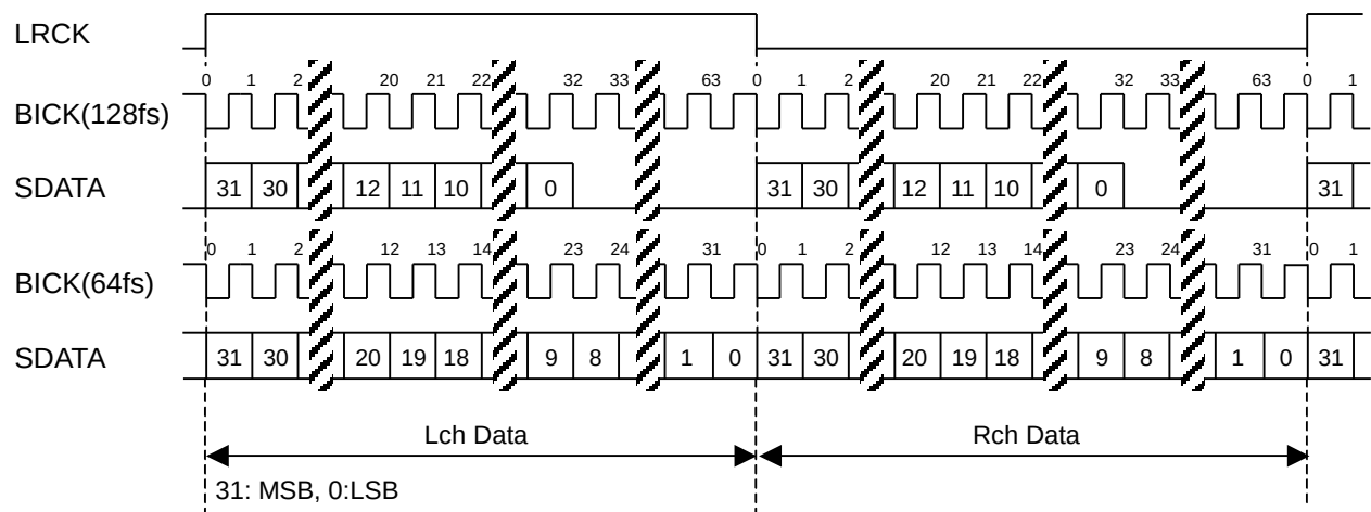
Figure 14. Mode 6 Timing
