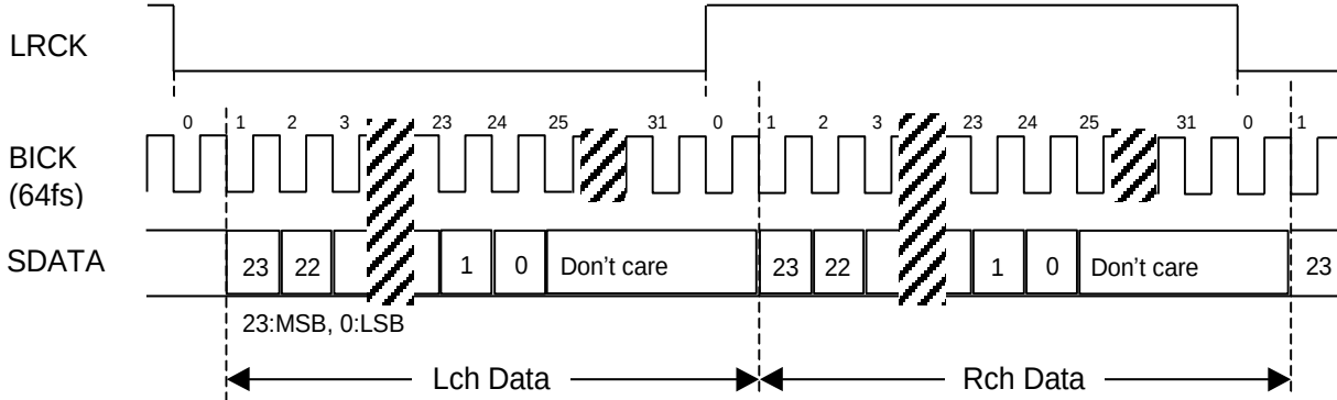
Figure 12. Mode 3 Timing
