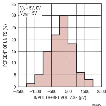
V_{OS} Distribution, V_{CM} = 5V (SOT-23, NPN Stage)
