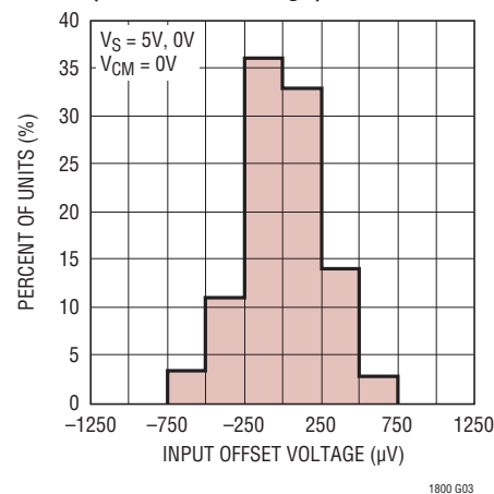
V_{OS} Distribution, V_{CM} = 0V (SOT-23, PNP Stage)
