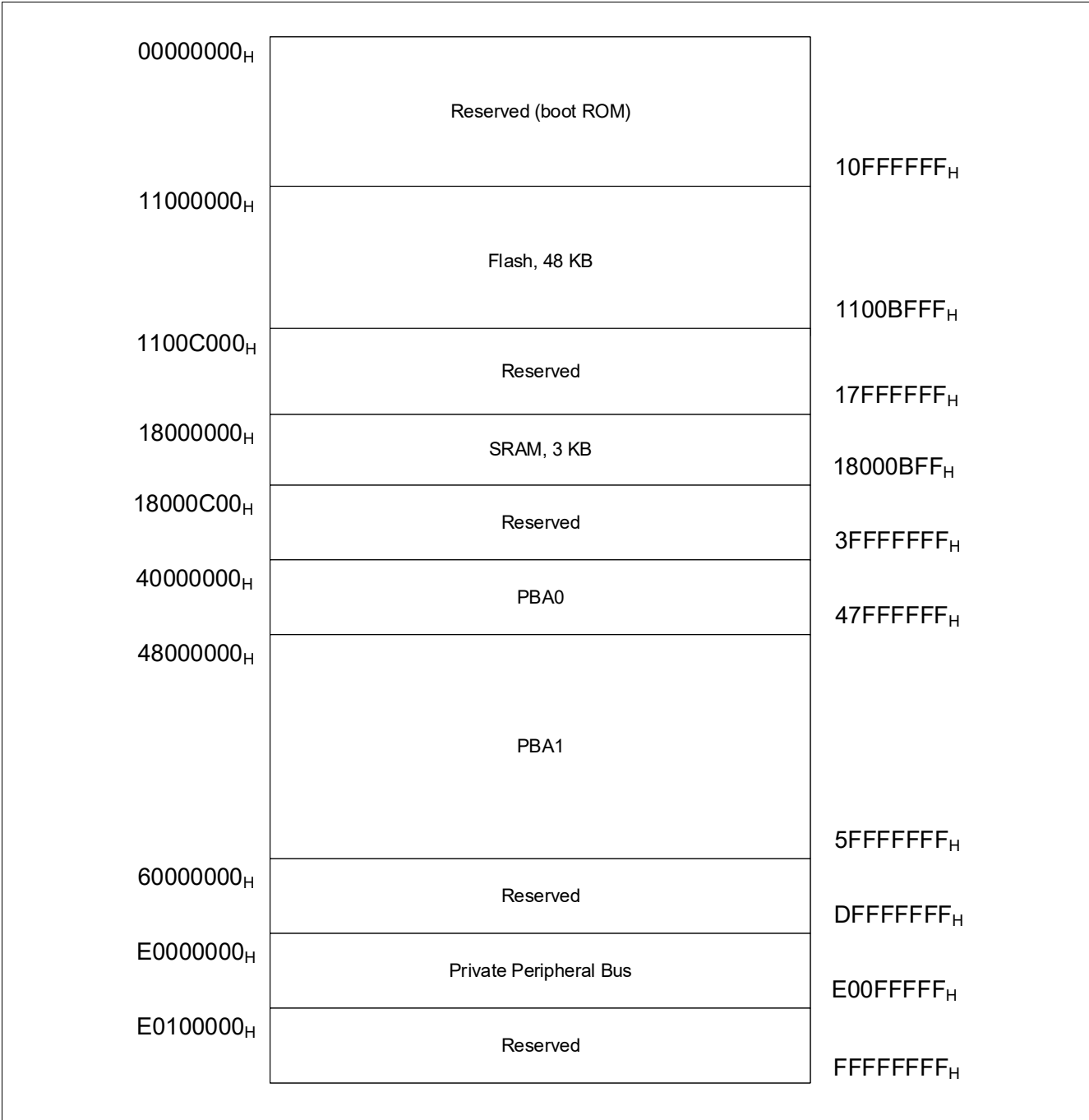
Figure 13 Memory map
