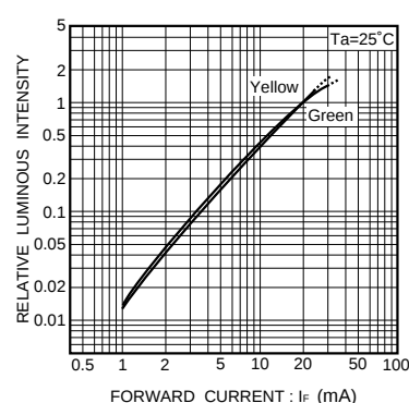
Fig. 25 Luminous intensity vs. forward current
