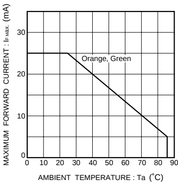
Fig. 22 Maximum forward current vs. ambient temperature
