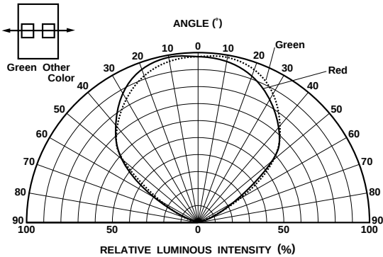
Fig. 1 Directional pattern (1)
