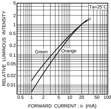
Fig. 19 Luminous intensity vs. forward current
