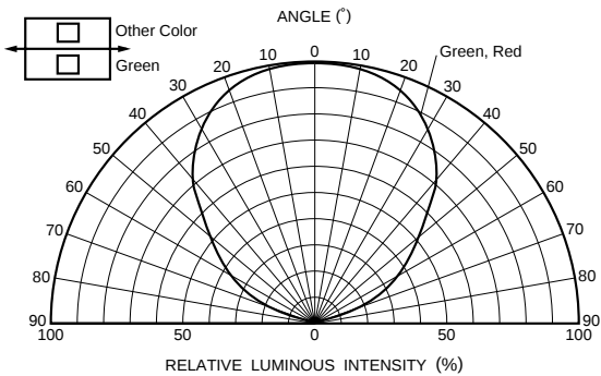
Fig. 2 Directional pattern (2)
