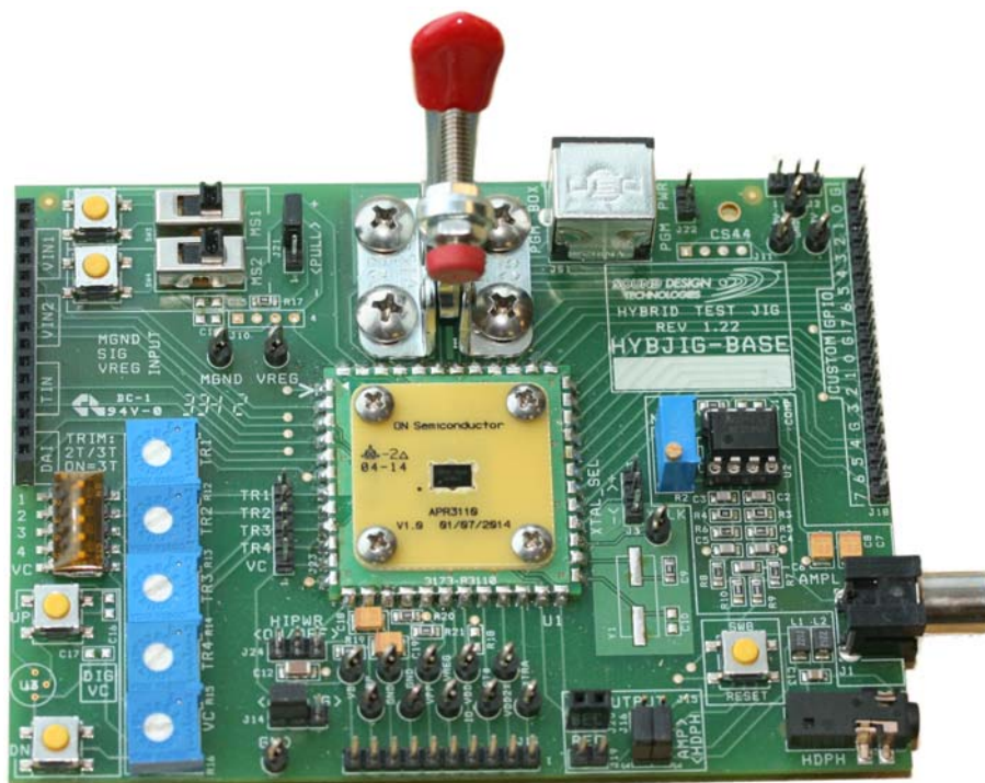
Figure 1. Hybrid Jig
