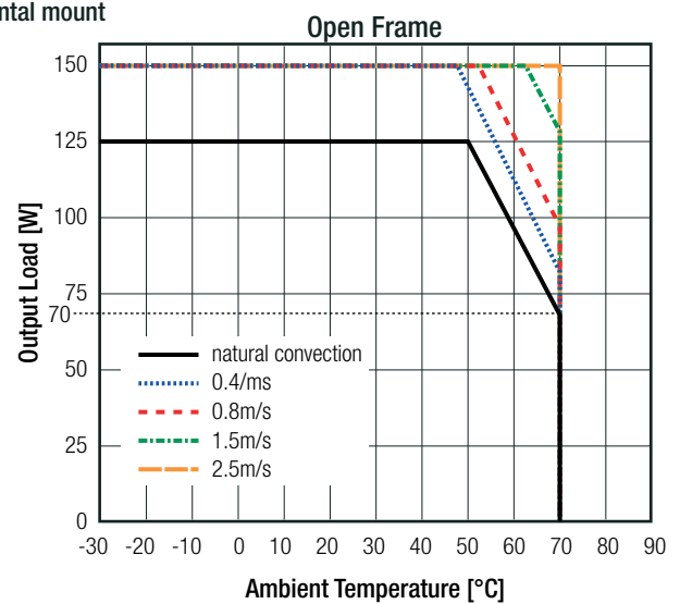
@ 115VAC, horizontal mount
