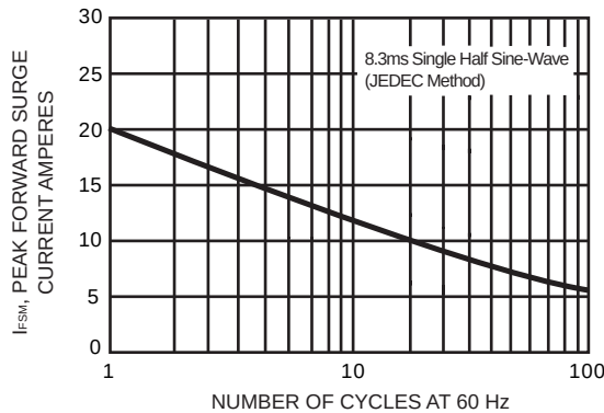
FIG. 5 MAXIMUM NON-REPETITIVE FORWARD SURGE CURRENT UNIDIRECTIONAL
