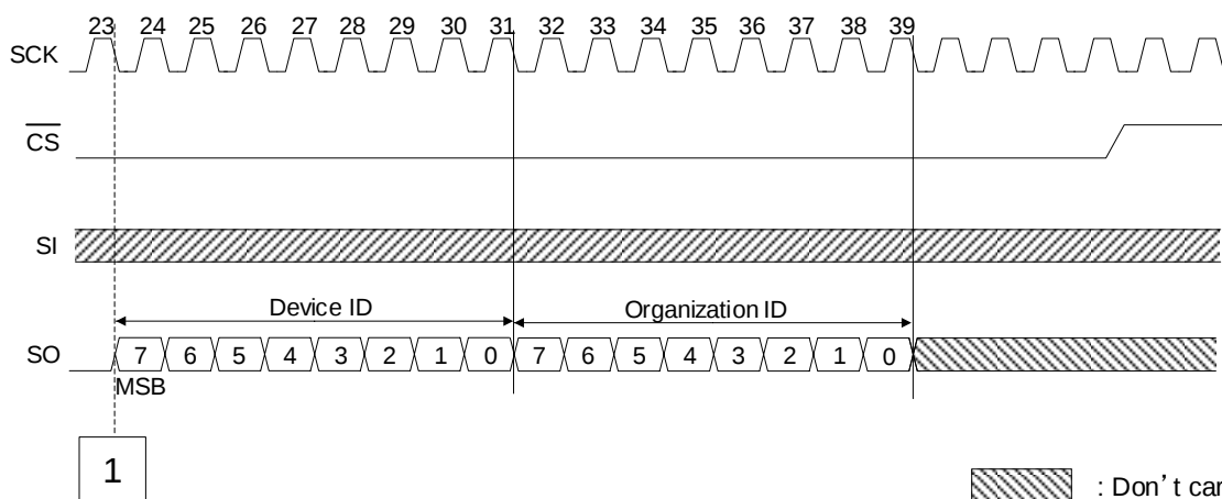
Figure 27. Read ID Timing
