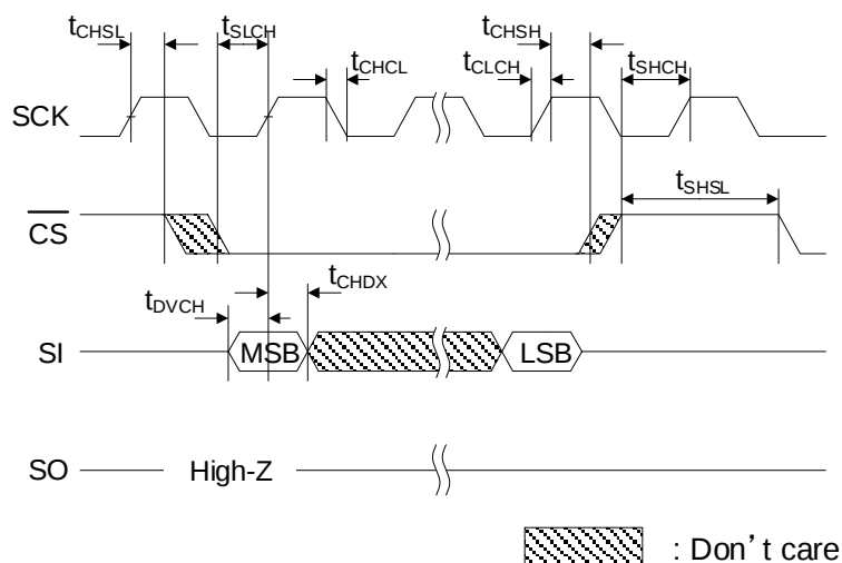
Figure 6. Serial Input Timing
