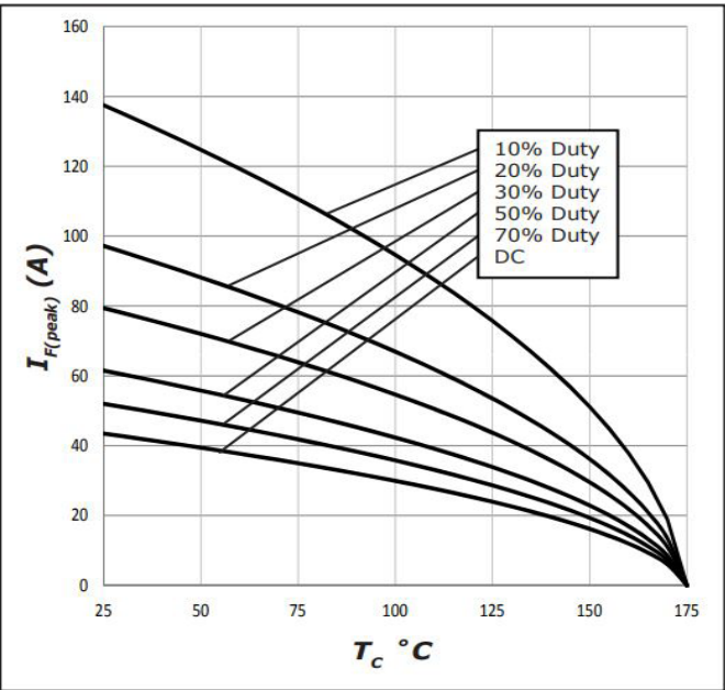
Figure 3 Current Derating
