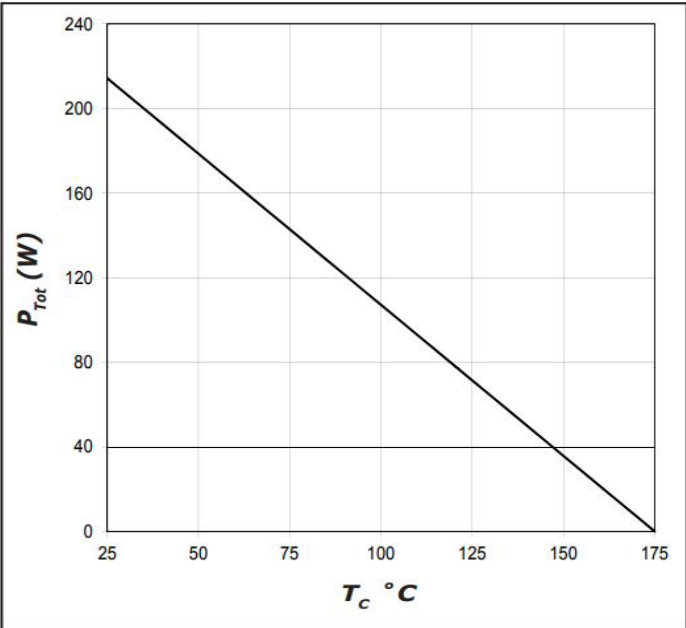
Figure 4 Power Derating
