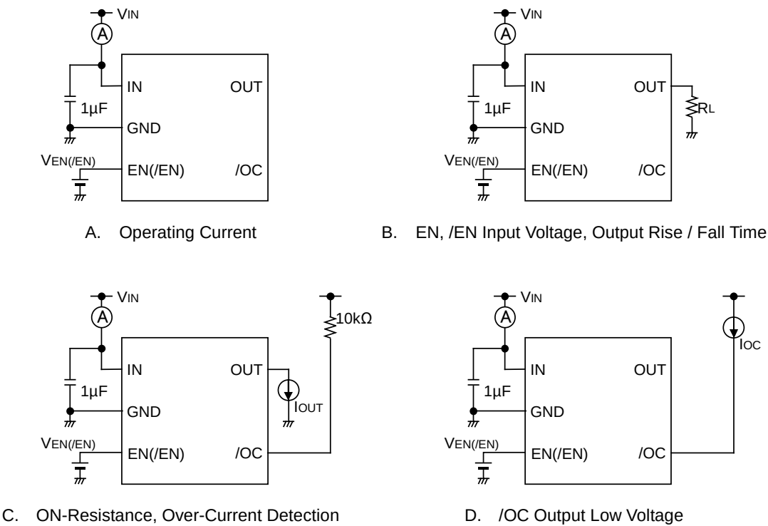
Figure 1. Measurement Circuit
