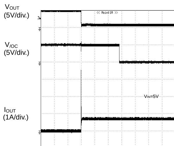
TIME (5ms/div.) Figure 78. Over-current response 1Ω load to enabled device
