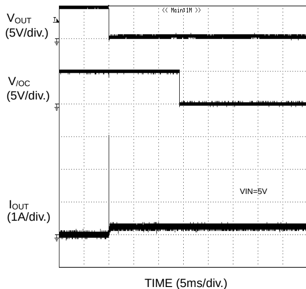
Figure 60. Over-Current Response 1Ω Load to Enabled Device
