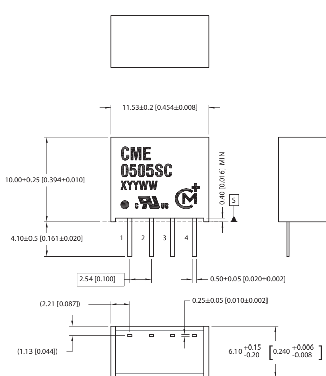
SC Package
