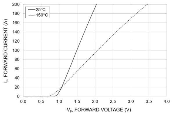
Figure 8. Buck Diode Forward Characteristics
