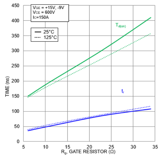
Figure 16. Typical Turn-On Switching Time vs. R g
