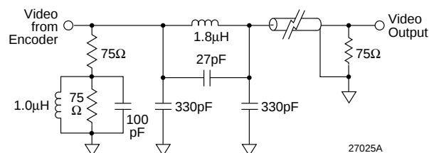
Figure 36. Recommended Output Reconstruction Filter
