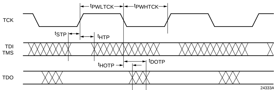
Figure 29. JTAG Test Port Timing
