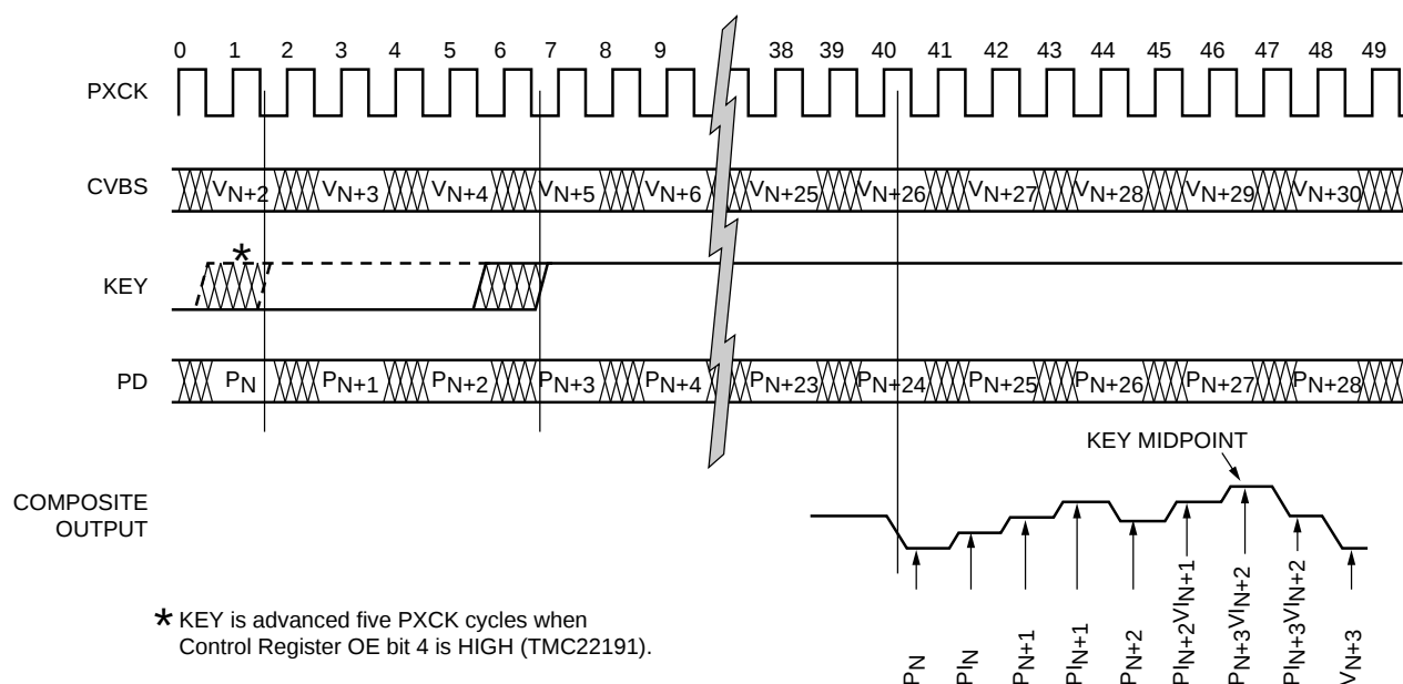
Figure 22. Hardware Keying
