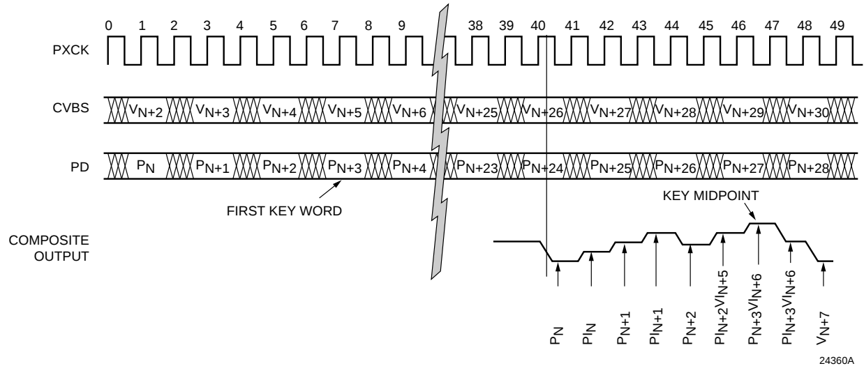
Figure 23. Data Keying
