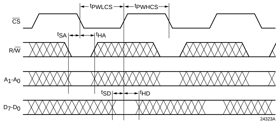
Figure 10. Microprocessor Port – Write Timing
