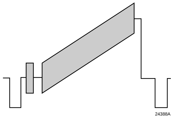
Figure 7. Modulated Ramp Waveform
