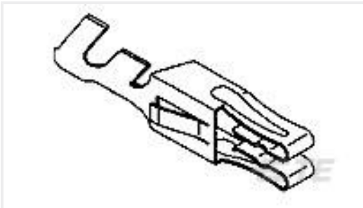
TE Part #5-530519-2 HIGH CURRENT CONT-STRIP
