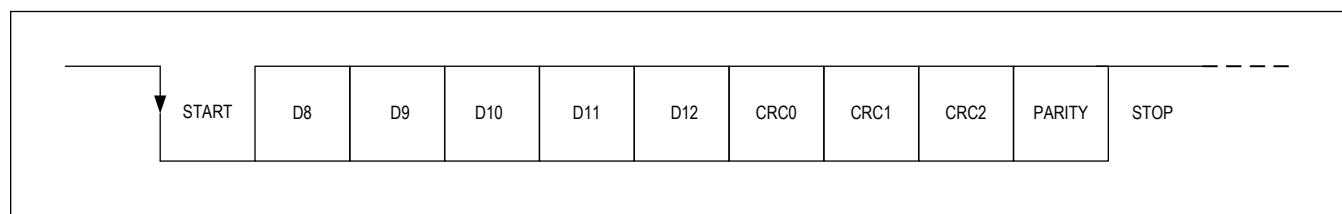
Figure 17. Final Frame
