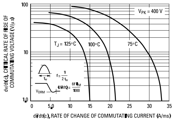
Figure 15. Critical Rate of Rise of Commutating Voltage
