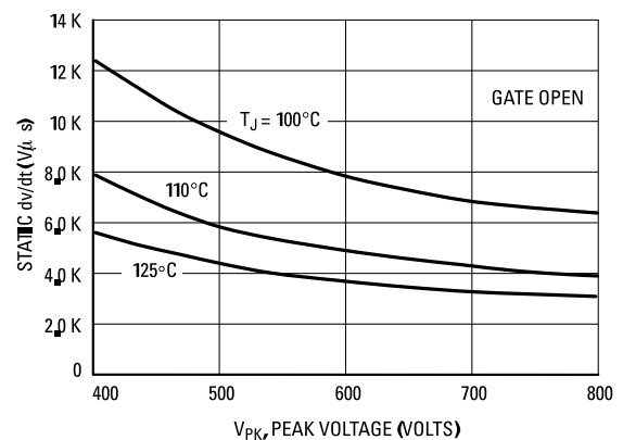
Figure 9. Exponential Static dv/dt vs. Peak Voltage, MT2(-)
