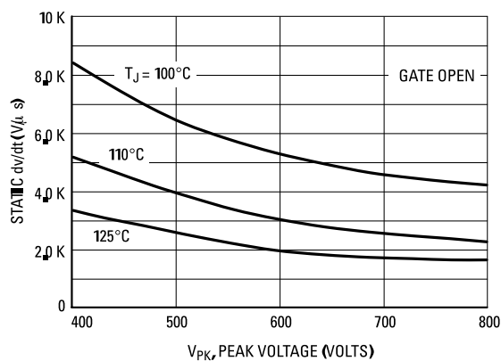
Figure 11. Exponential Static dv/dt vs. Peak Voltage, MT2(+)
