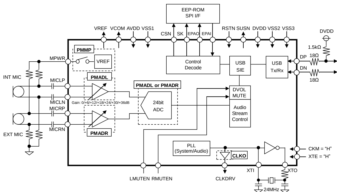
Figure 1. Block Diagram
