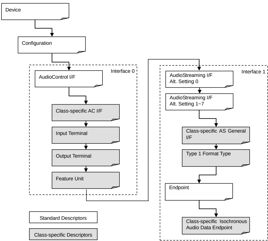
Figure 17. Descriptor Hierarchy
