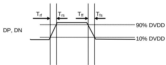
Figure 4. Rise/Fall Time
