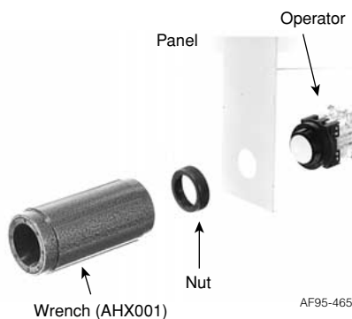
Fig. 2 Pushbutton with a round bezel
