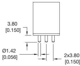
SIZE 18 CONTACTS
