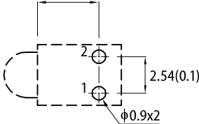
Recommended PCB Layout 4.08(0.161)Typ.
