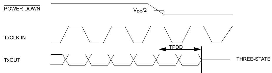
Figure 12. Transmitter power-down delay
