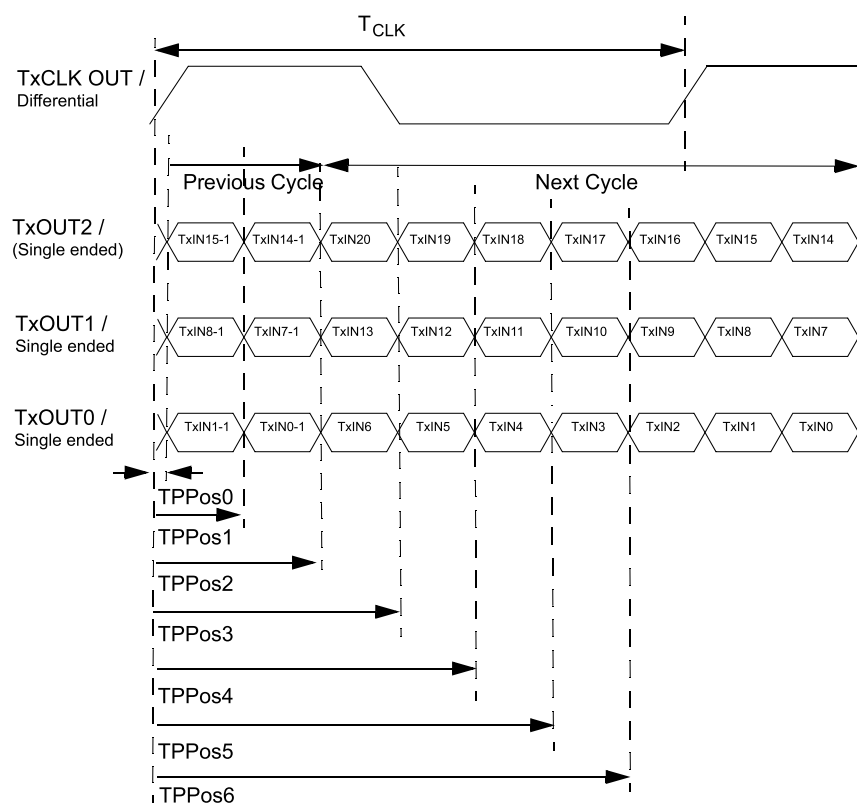
Figure 13. RHFLVDS217 output pulse position measurement
