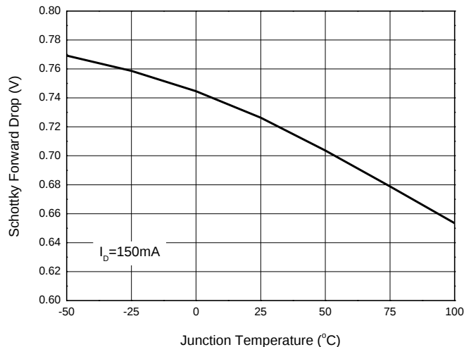
Schottky Forward Drop vs. Junction Temperature
