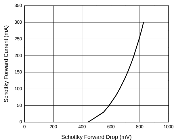
Schottky Forward Current vs. Schottky Forward Drop
