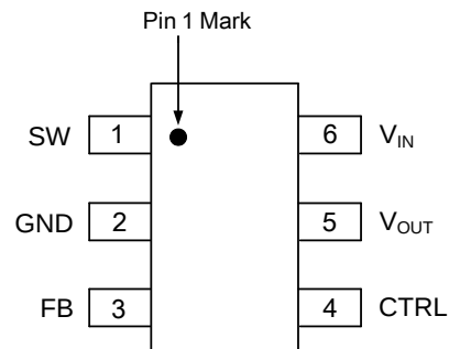
K/KT Package (SOT-23-6/TSOT-23-6)
