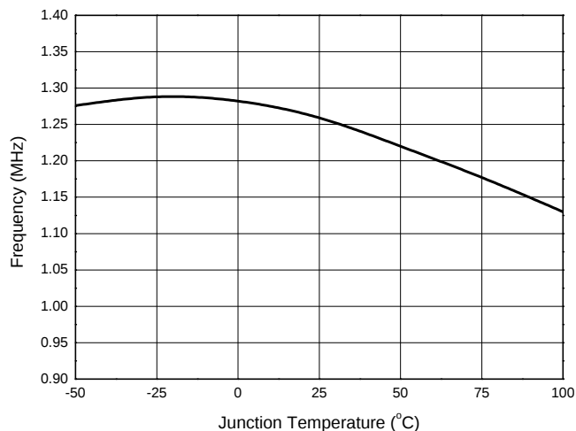
Frequency vs. Junction Temperature
