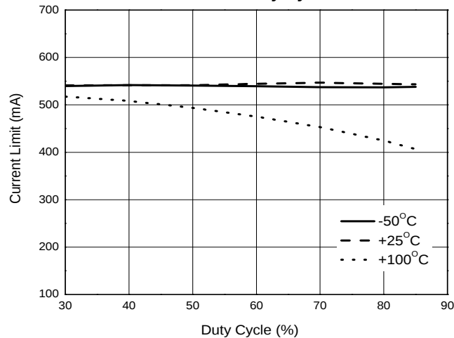
Current Limit vs. Duty Cycle
