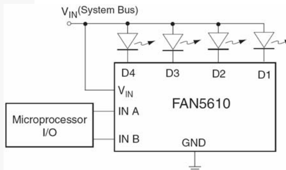
Figure 13. Drive High V_F White or Blue LEDs from Existing Bus from 4.0V to 5.5V
