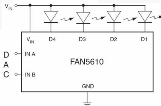
Typical Application
