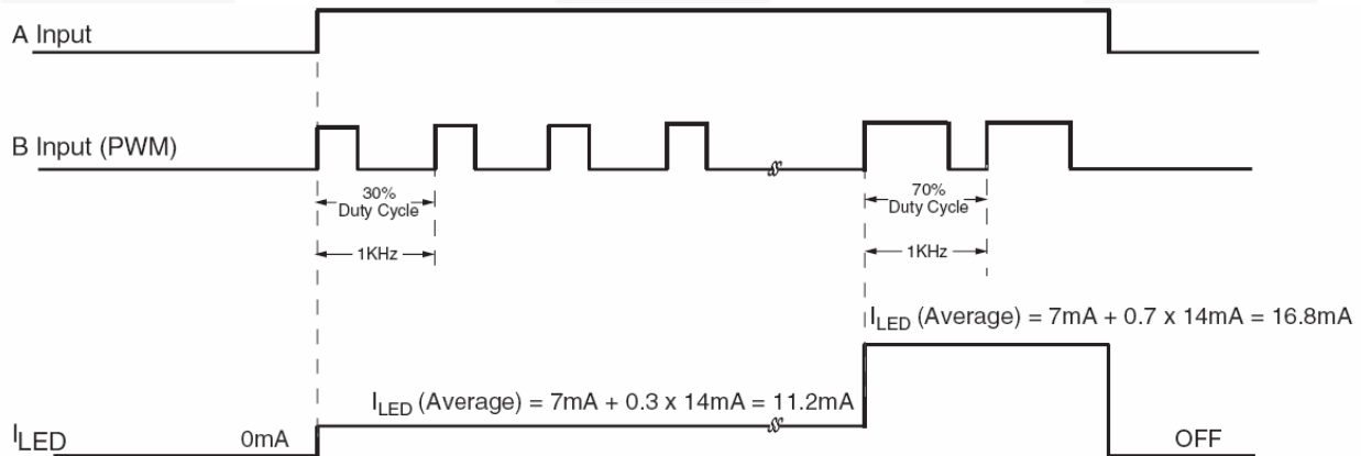
Figure 9. A is HIGH and B is PWM. I_{\text{LED}} (\text{average}) = 7\text{mA} + \delta \times 14\text{mA} , where \delta is duty cycle. (3,4)
