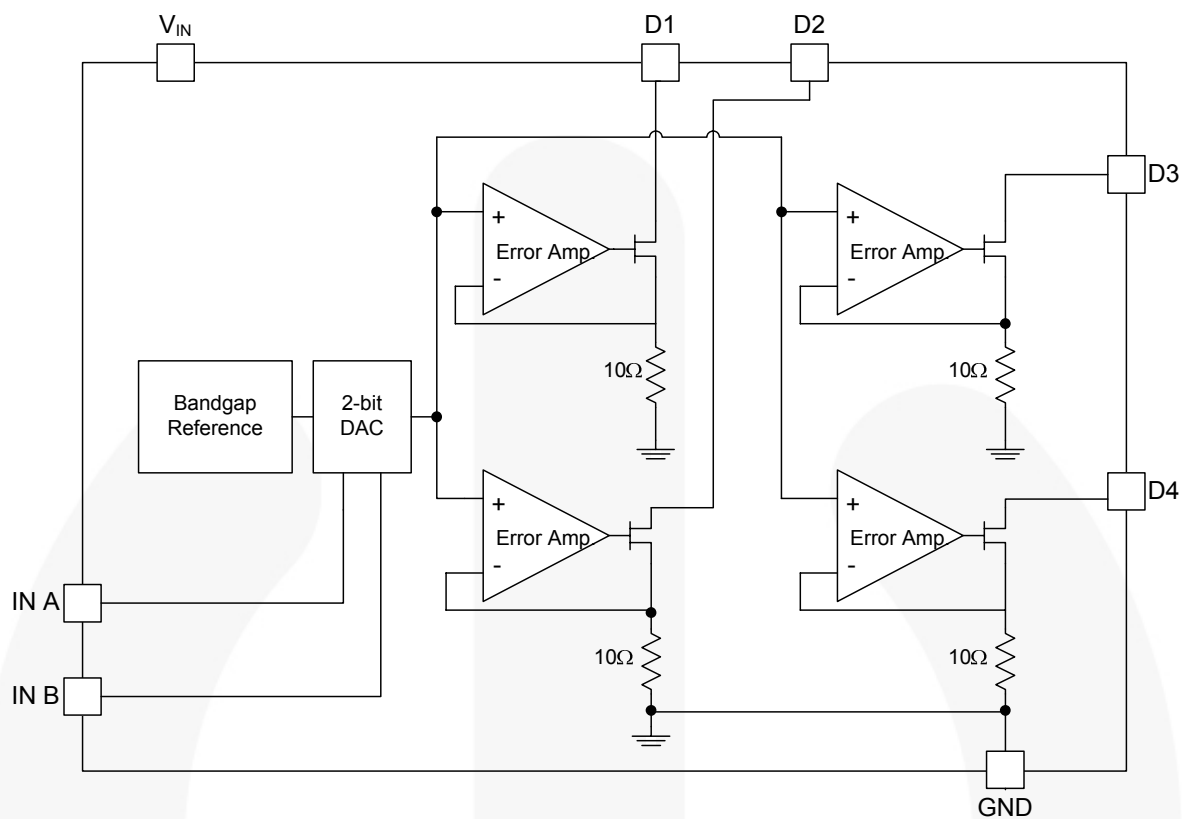
Figure 2. Block Diagram
