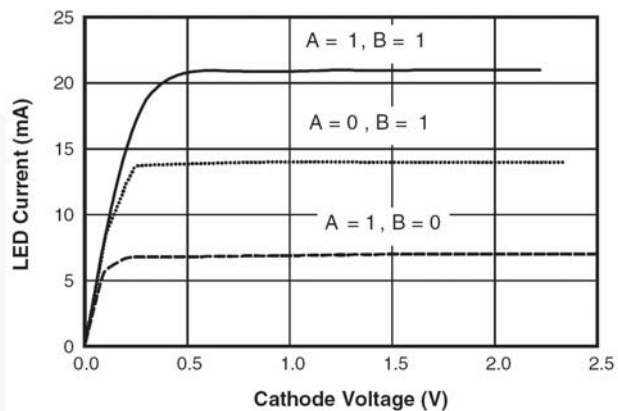
Figure 4. LED Current vs. Cathode Voltage
