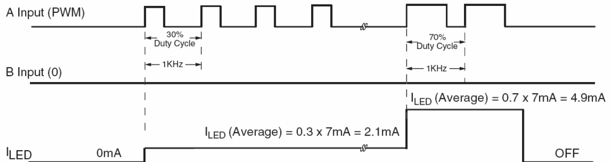
Figure 8. A is PWM and B is LOW. I_{\text{LED}} (\text{average}) = \delta \times 7\text{mA} , where \delta is duty cycle. (2)
