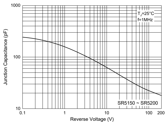
Fig. 12 - Typical Capacitance Characteristics
