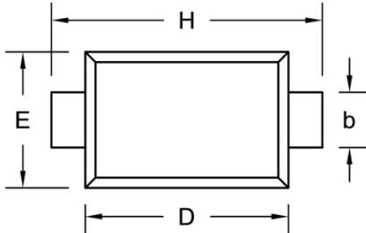
SOD-523F
