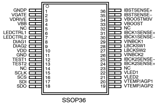
Figure 2. Pin Connections
