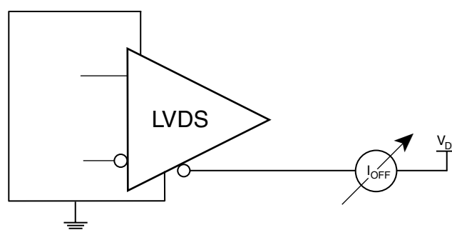
POWER OFF LEAKAGE
