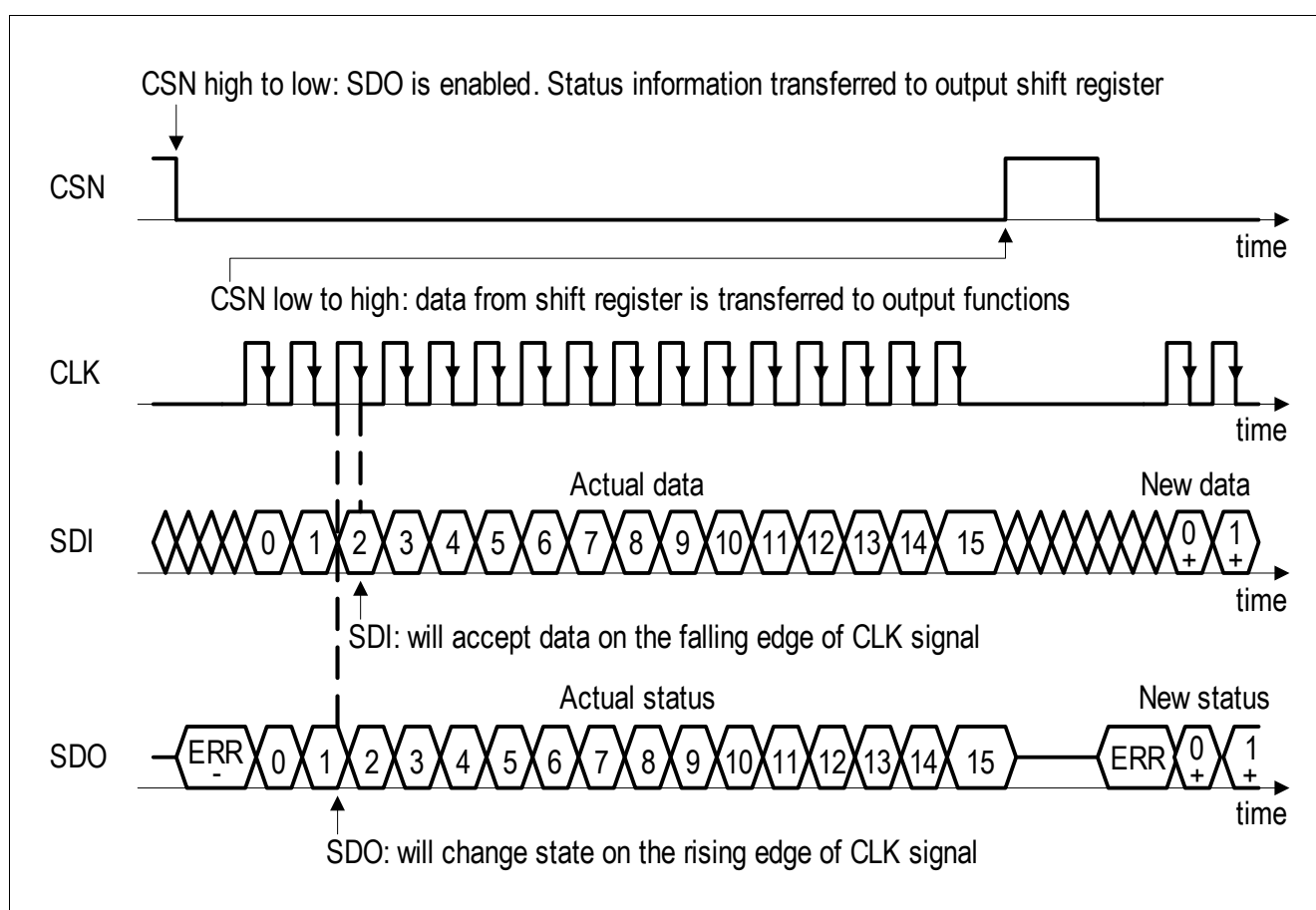
Figure 46 SPI data transfer timing (note the reversed order of LSB and MSB shown in this figure compared to the register description)
