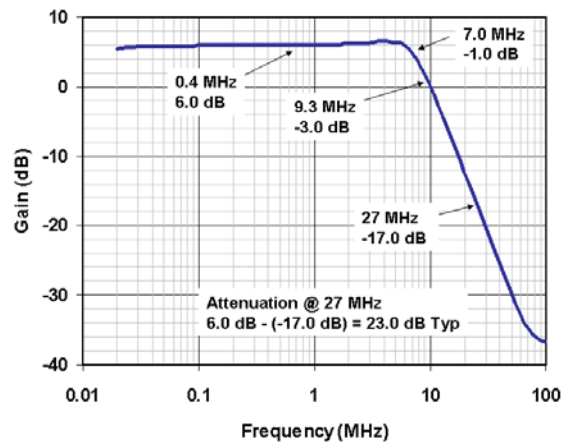
Figure 2. Frequency Response
