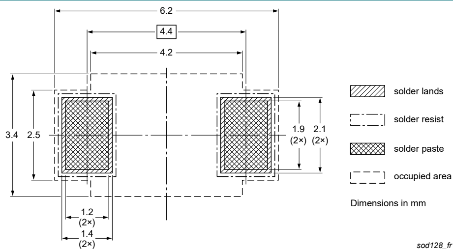
Fig. 11. Reflow soldering footprint for CFP5 (SOD128)
