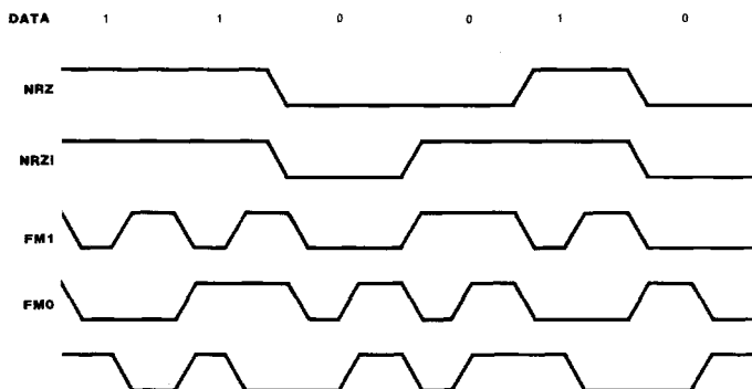
Figure 6. Data Encoding Methods
