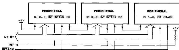
Figure 7. Interrupt Schedule
