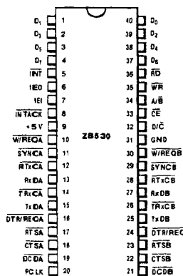
Figure 2a. DIP Pin Assignments, Z8530
