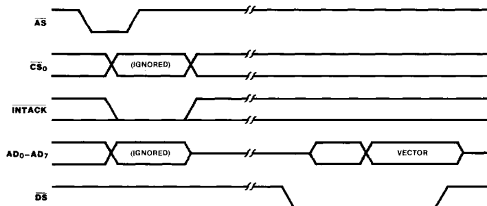
Figure 17. Interrupt Acknowledge Cycle Timing
