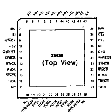
Figure 2d. Chip Carrier Pin Assignments, Z8030
