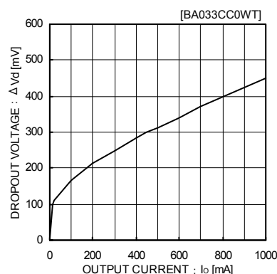
Fig.5 Input/Output Voltage Difference ( I_{OUT}(0V=1A) )
