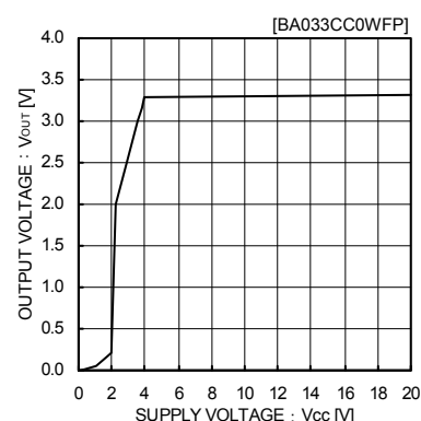
Fig.3 Input Stability ( I_O=500mA )
