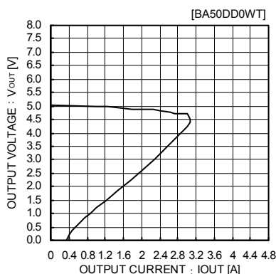
Fig.16 Load Stability
