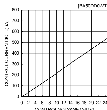
Fig.21 CTL Voltage vs. CTL Current
