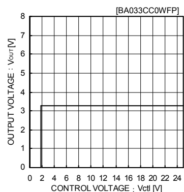
Fig.10 CTL Voltage vs. Output Voltage
