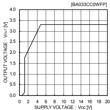
Fig.2 Input Stability
