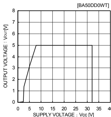
Fig.23 Overvoltage Operating
