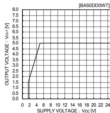
Fig.15 Input Stability ( I_O=2A )
