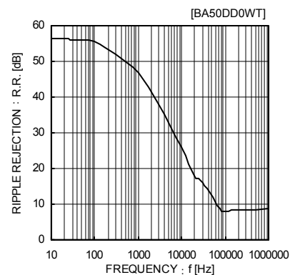
Fig.18 Ripple Rejection Characteristics
