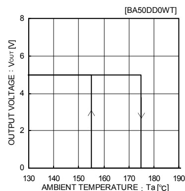
Fig.24 Thermal Shutdown Circuit Characteristics
