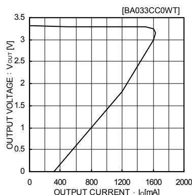
Fig.4 Load Stability
