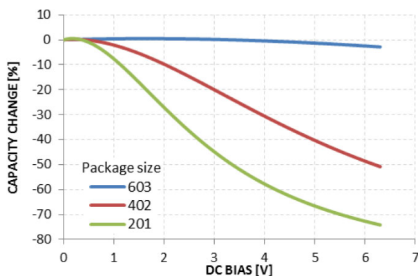
Figure 24. Capacity vs. DC Bias Voltage
