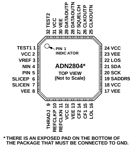
Figure 5. Pin Configuration
