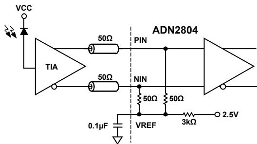
Figure 27. DC-Coupled Application
