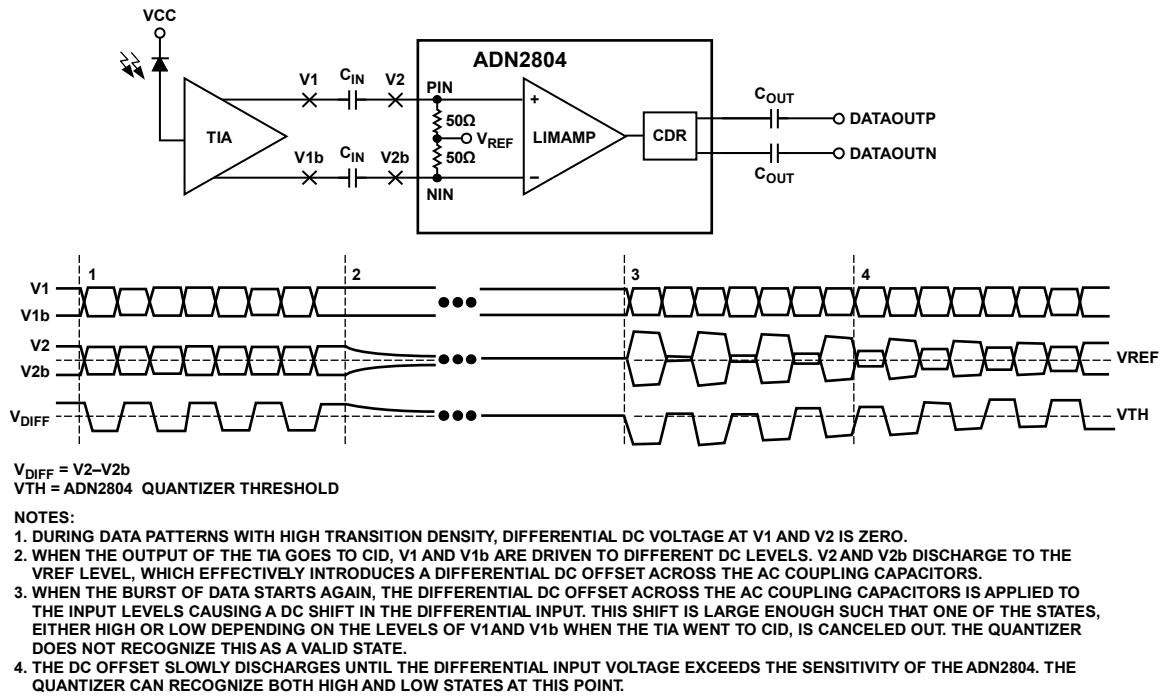
Figure 26. Example of Baseline Wander
