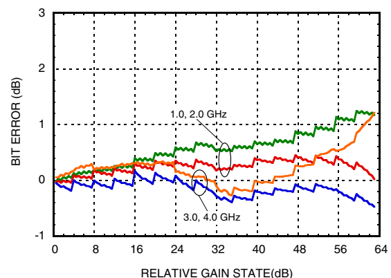
Bit Error vs. Relative Gain State [1]
