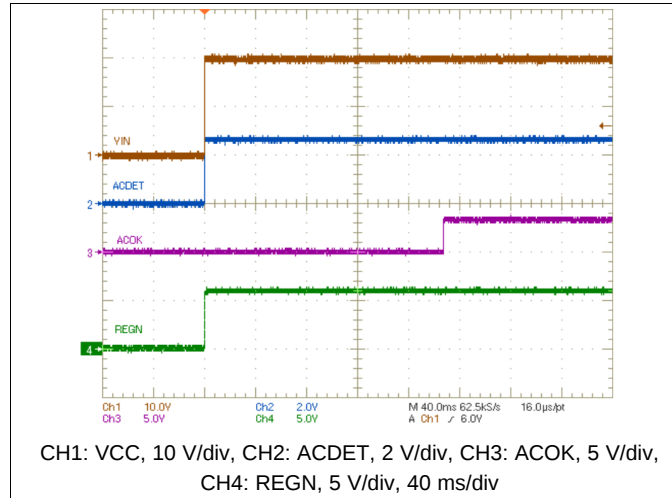
Figure 1. VCC, ACDET, REGN and ACOK Power Up
