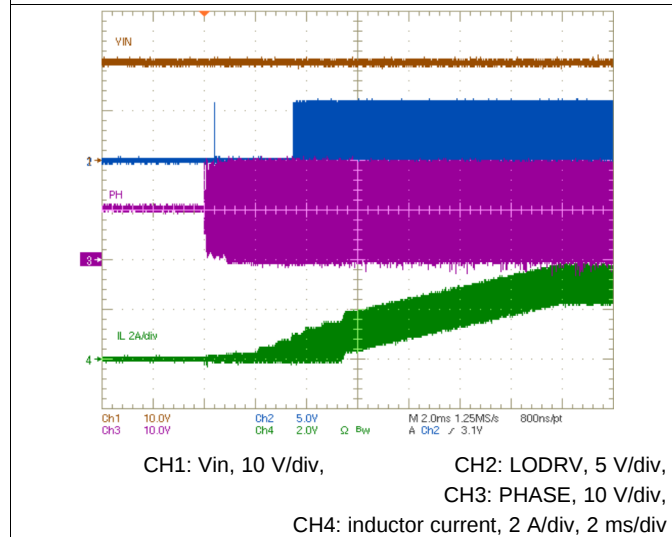
Figure 3. Current Soft-Start
