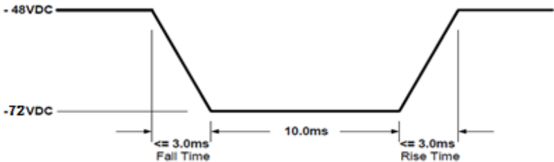
Figure 4. Minus 72 VDC Line Transient Test
