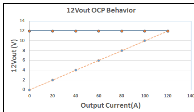
Figure 7. Current Limitation on V_I
