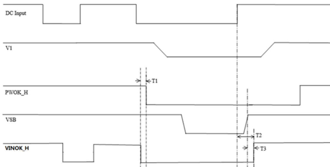
Figure 13. VINOK_H Timing
