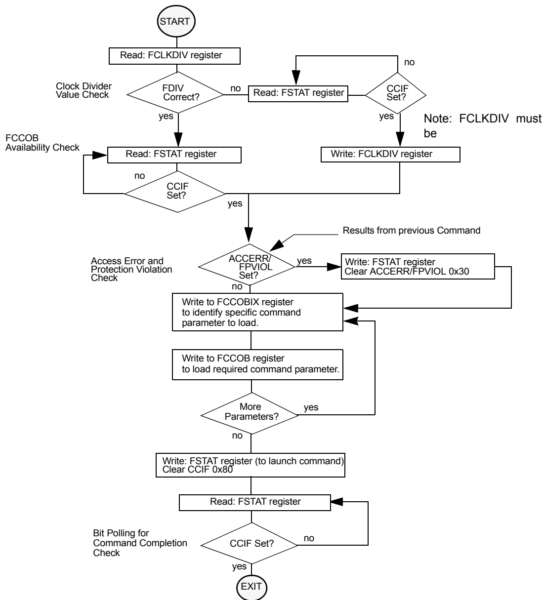
Figure 109. Generic Flash Command Write Sequence Flowchart
