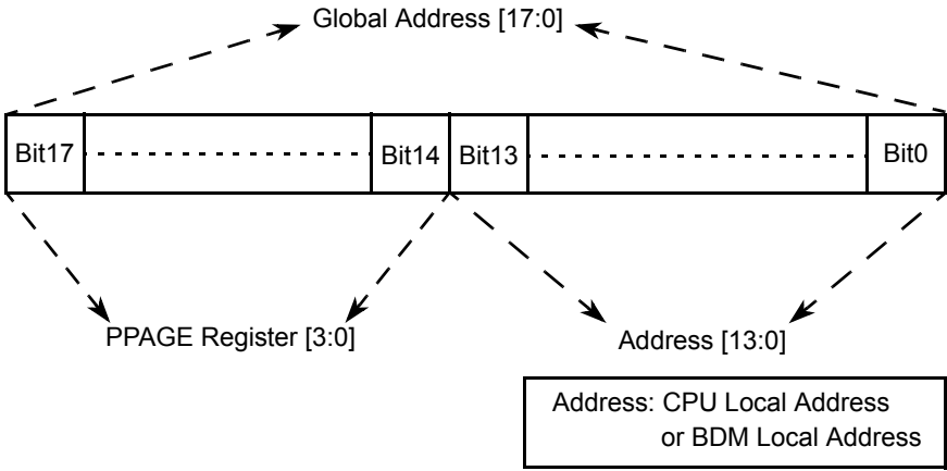
Figure 49. PAGE Address Mapping
