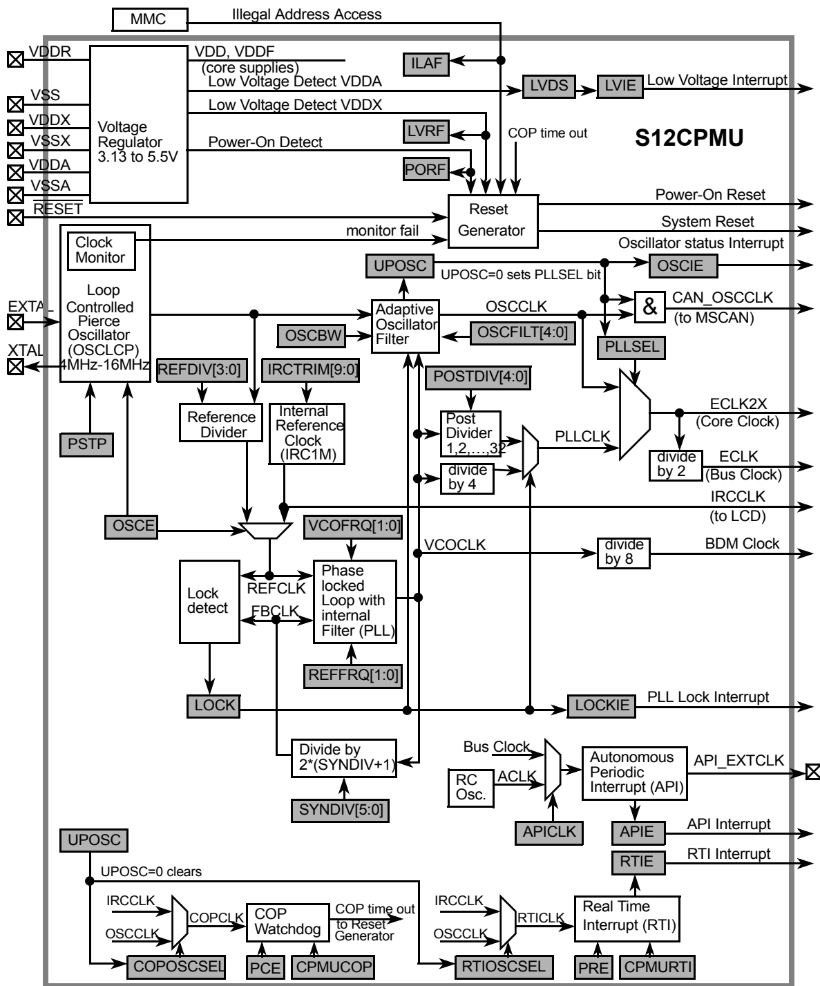
Figure 84. Block diagram of S12CPMU
