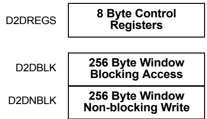
Figure 112. D2DI Top Level Memory Map
