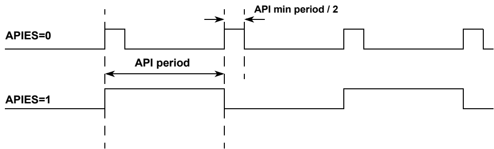
Figure 86. Waveform selected on API_EXTCLK pin (APIEA=1, APIFE=1)
