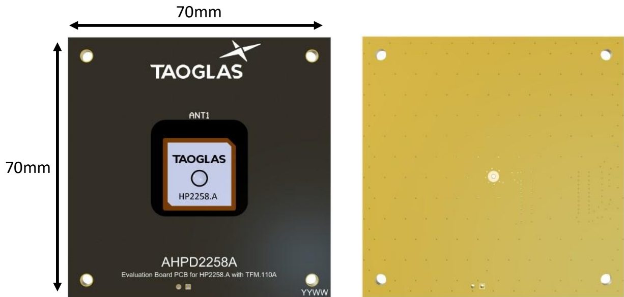
Top Side (70x70mm example PCB Reference Design)
