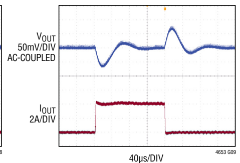
1V Transient Response, 24V_{IN}
