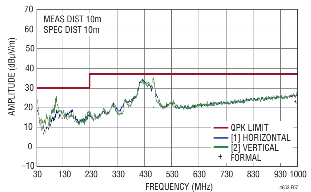
Figure 7. Radiated Emissions Scan of the LTM4653 Producing 24V OUT at 3.5A, from 48V IN , DC2327A Hardware, f_{SW} = 1.2\text{MHz} , Measured in a 10m Chamber, Peak Detect Method
