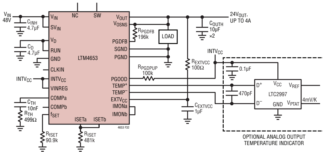
Figure 32. 4A, 24V Output DC/DC \mu Module Regulator
