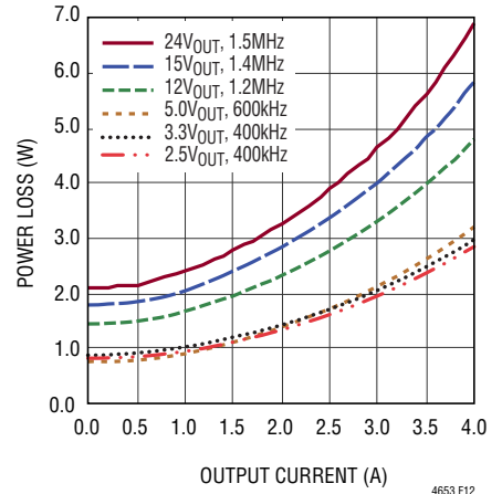
Figure 12. 48VIN Power Loss Curve
