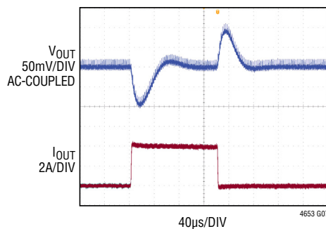
3.3V Transient Response, 48V_{IN}
