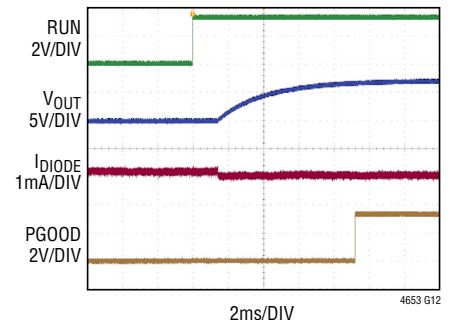
Start-Up, Pre-Bias
