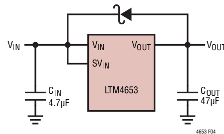
Figure 4. Schottky Diode from V_{OUT} to V_{IN}
