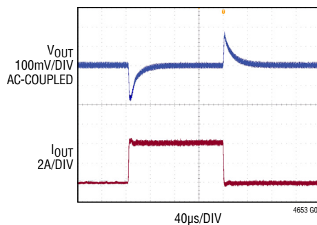
12V Transient Response, 48V_{IN}
