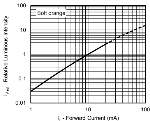
Fig. 10 - Relative Luminous Intensity vs. Forward Current
