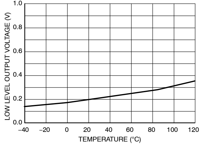
Figure 28. Low Level Output Voltage vs. Temperature
