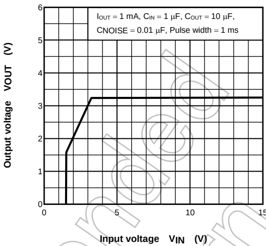
(TAR5S33) V_{OUT} - V_{IN}
